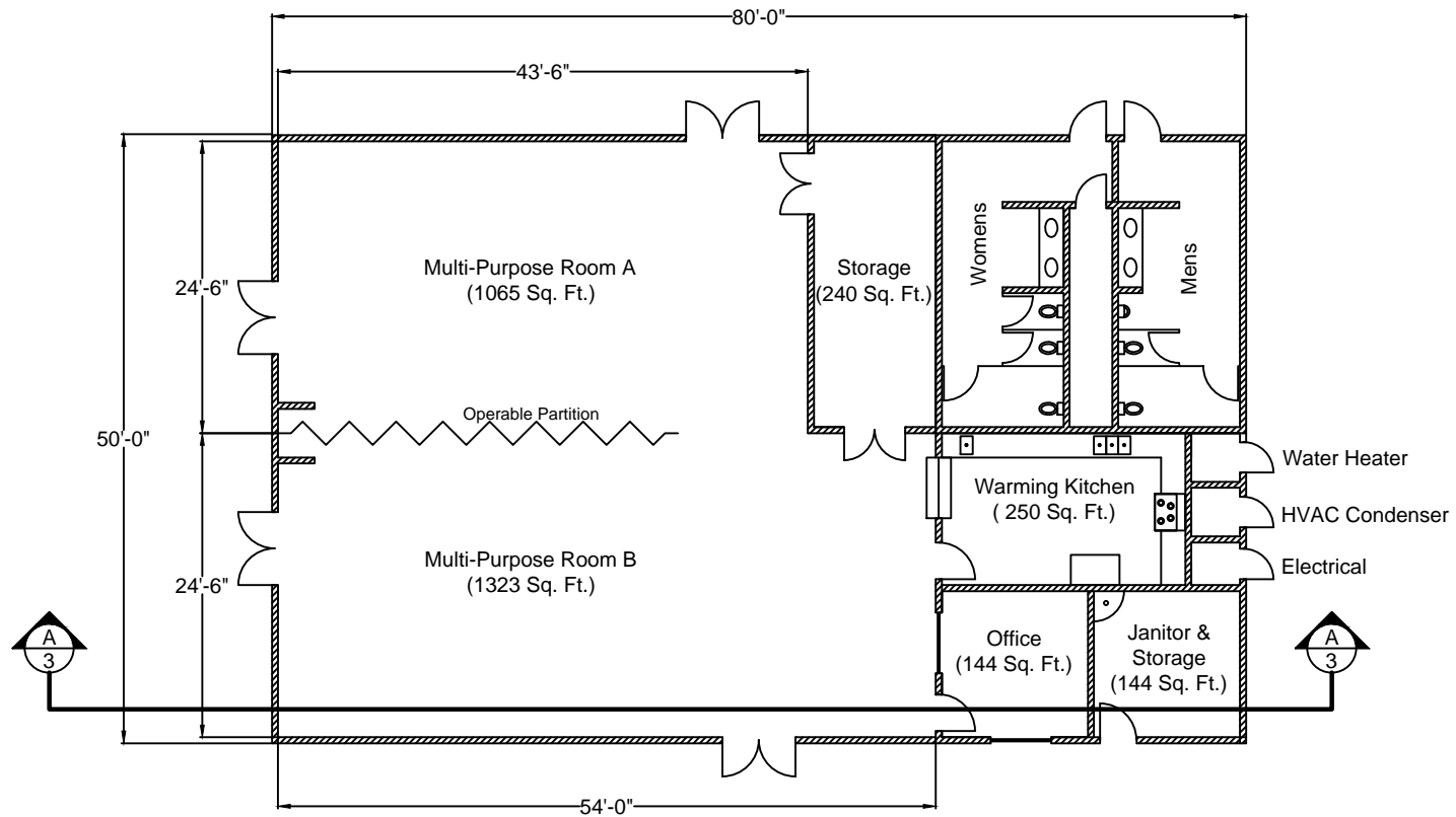
Floor Plan - 4000 Sq.Ft. Scale 1" = 16'-0"
